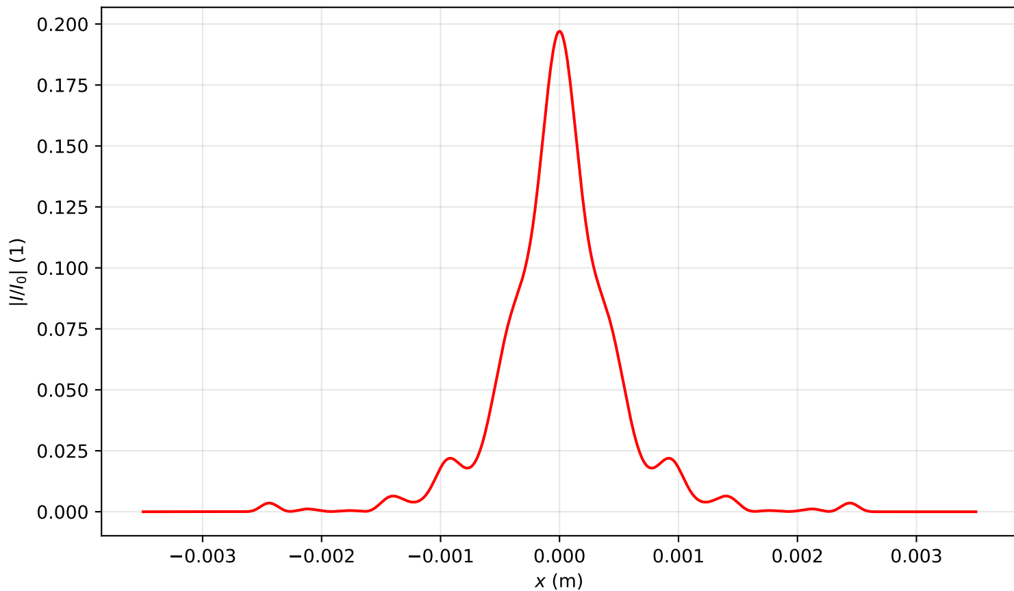
Intensity profile I(x, y = 0, z = 3.184)/I_0 , \text{Pin}=5.0\text{Pcr} , artificial time
